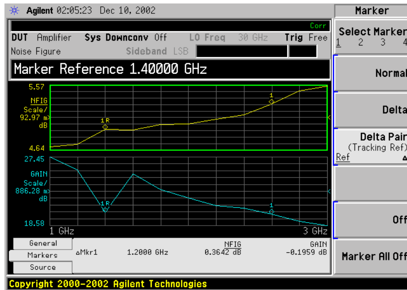
Figure 2-15 Delta Pair with Reference Marker Enabled
