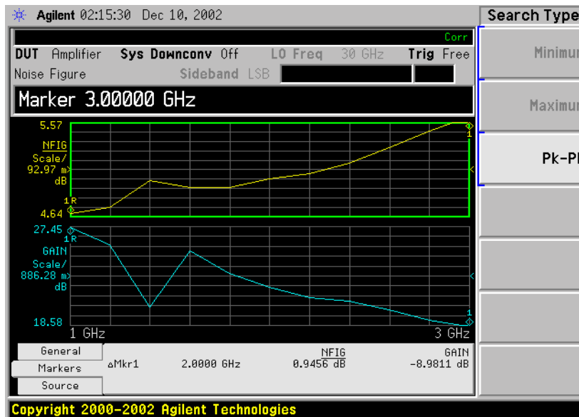
Figure 2-18 Peak to Peak Found
