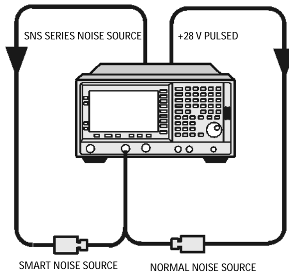
Figure 2-19 ESA Calibration Setup with Normal or Smart Noise Sources
