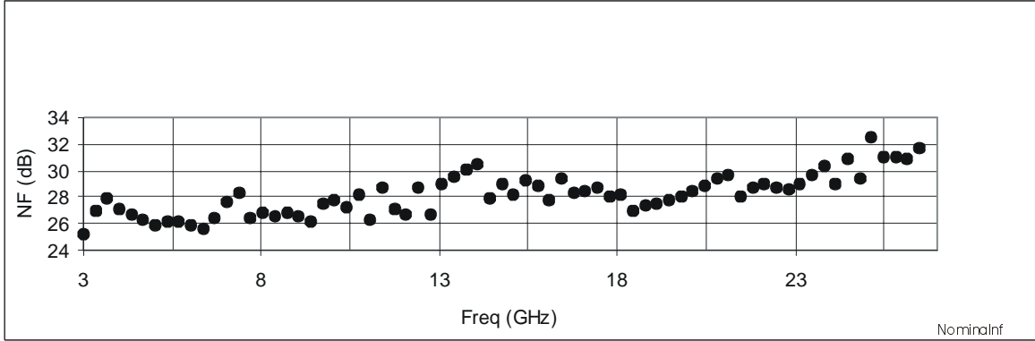
Figure 8-3 No Preamp - Nominal Noise Figure 1
