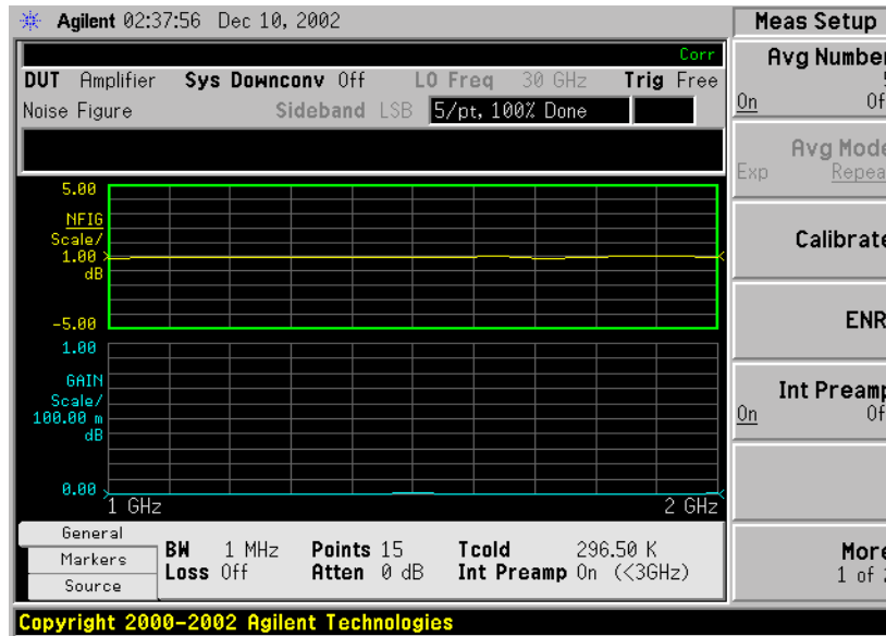
Figure 2-21 Typical Graph after calibration is complete
