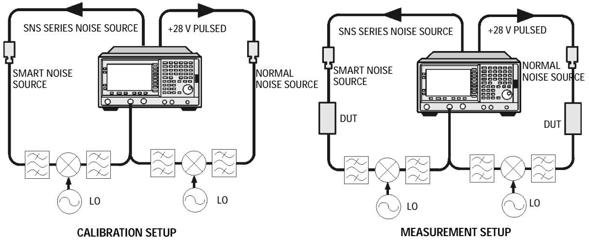
Figure 4-4 Setting Up a PSA for Frequency Converting DUT Measurement
