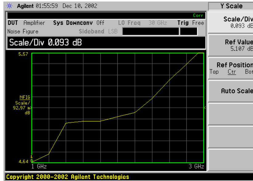
Figure 2-11 Typical Noise Figure Displayed on a Graph
