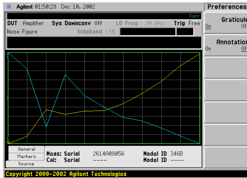
Figure 2-10 Typical Graph with Annotation Switched Off
