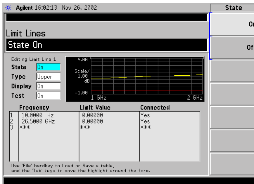
Limit Line Table before Limit Lines Values are Added
