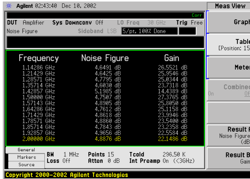
Figure 2-25 Typical Tabulated Results after Measurement
