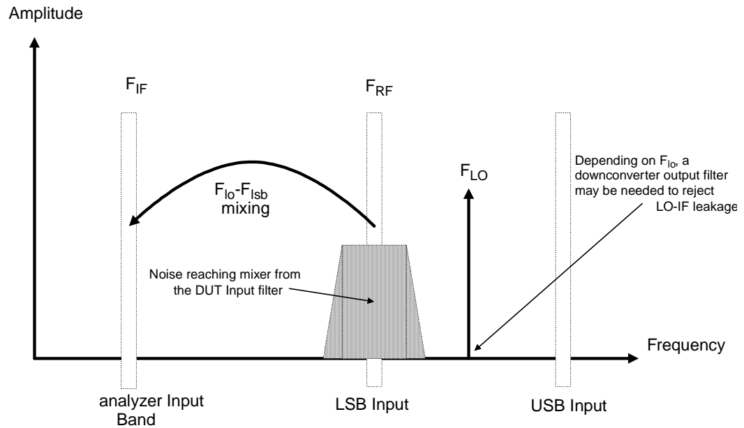
Figure 4-20 LSB System Downconverter Measurements
