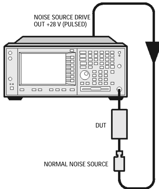
Figure 2-24 Connecting the DUT to make a measurement on a PSA
