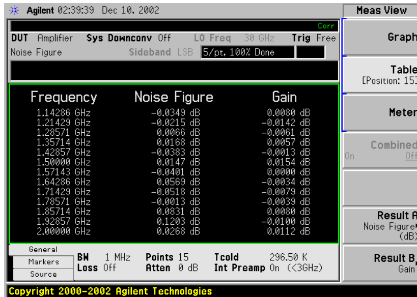
Figure 2-22 Typical Tabulated Results after Calibration
