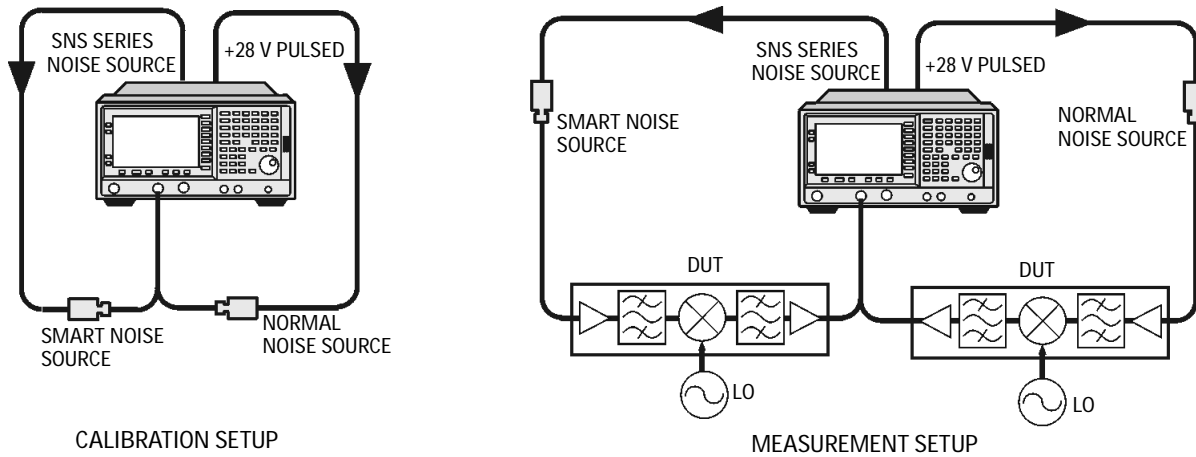
Figure 4-13 ESA Frequency Converting DUT Calibration and Measurement
