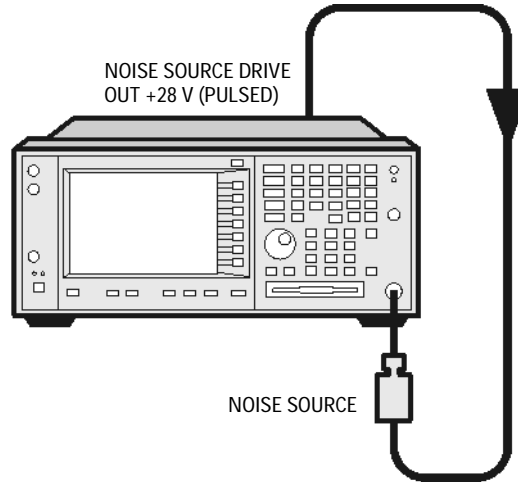
Figure 2-20 PSA Calibration Setup with Normal Noise Source
