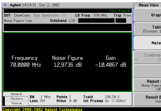
Figure 4-16 Typical Microwave Results
