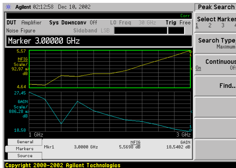
Figure 2-17 Typical Trace showing Maximum Point Found
