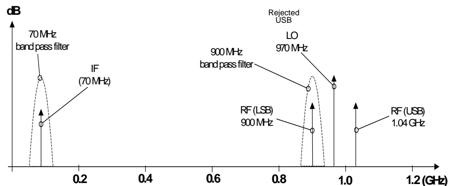
Figure 4-11 Fixed LO (970 MHz) and Fixed IF (70 MHz), LSB Spectrum
