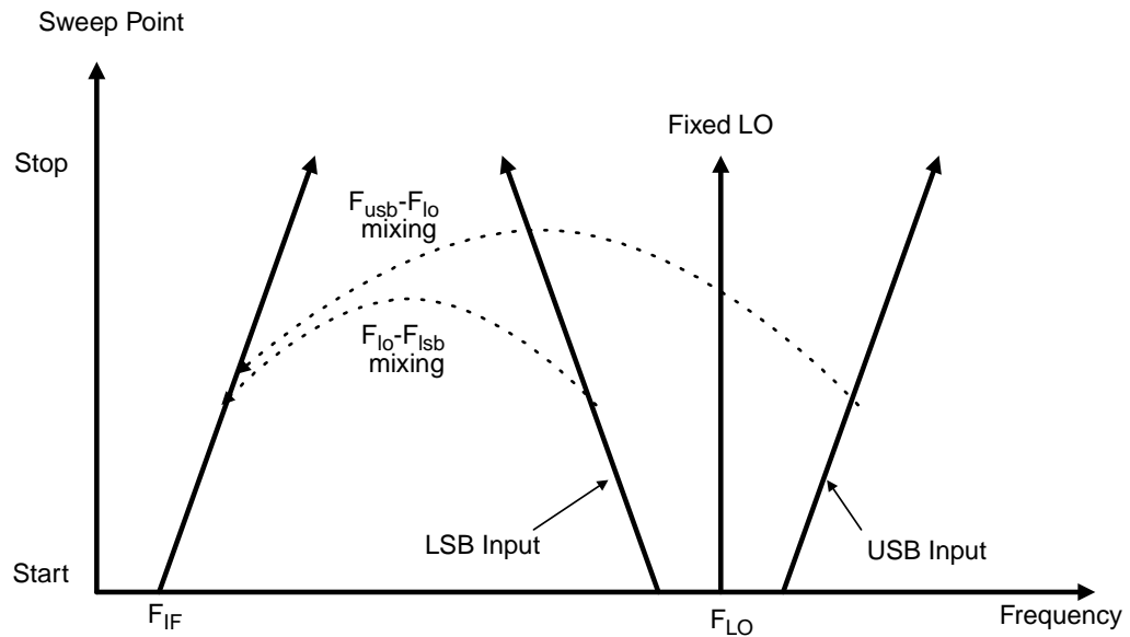
Figure 4-10 Fixed LO Measurements
