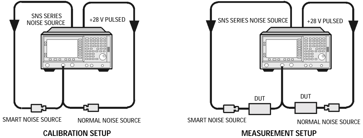
Figure 4-1 ESA Basic Noise Figure Measurement - No Frequency Conversion
