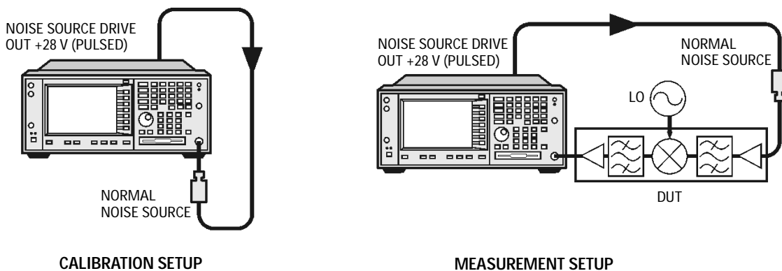
Figure 4-6 PSA Frequency Converting DUT Measurement
