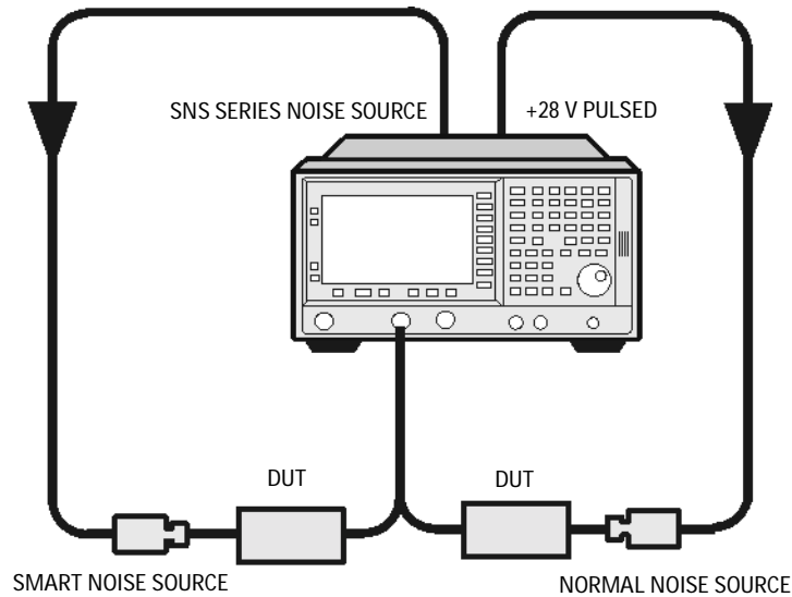
Figure 2-23 Connecting the DUT to make a measurement on an ESA
