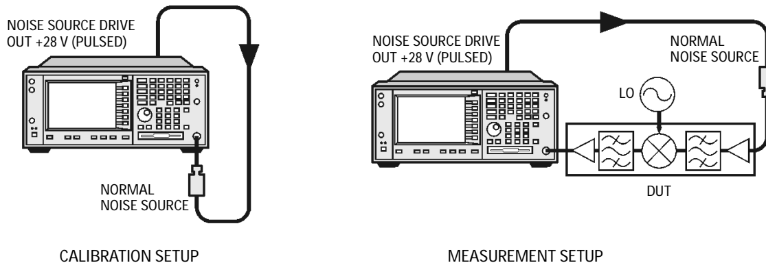
Figure 4-14 PSA Frequency Converting DUT Calibration and Measurement
