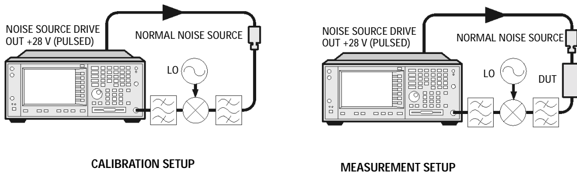
Figure 4-18 PSA System Downconverter Calibration and Measurement
