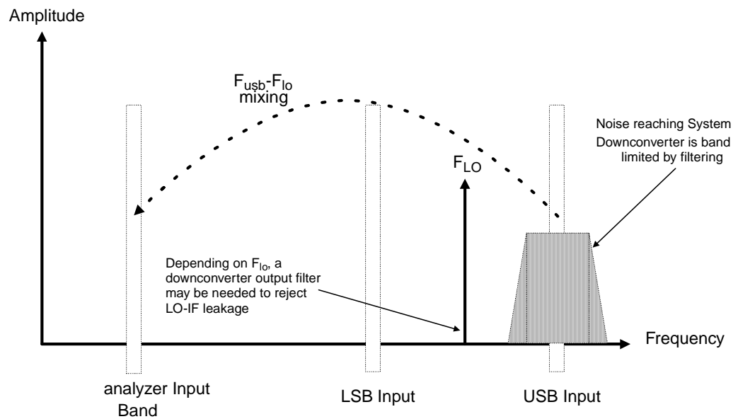
Figure 4-21 USB System Downconverter Measurements
