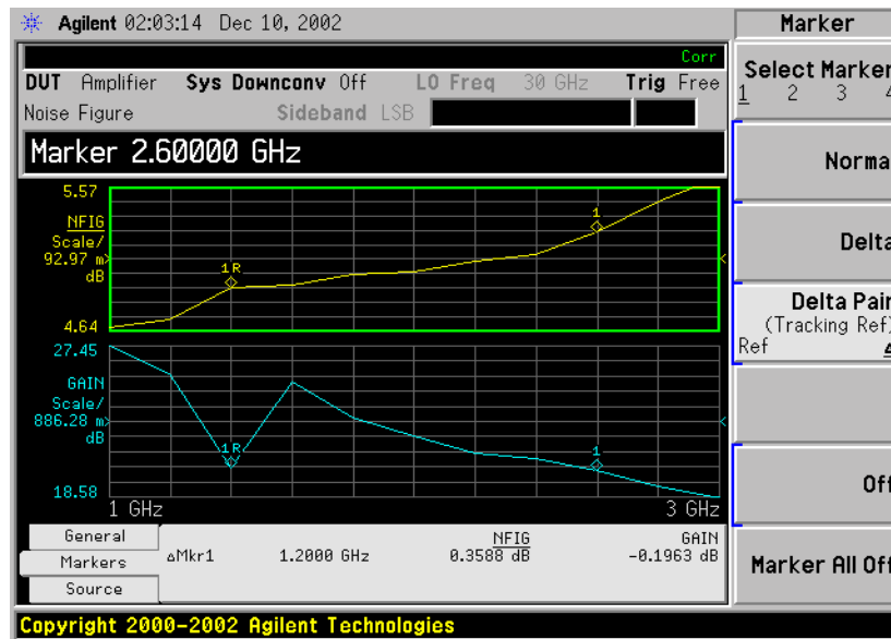
Figure 2-16 Delta Pair with Delta Marker Enabled
