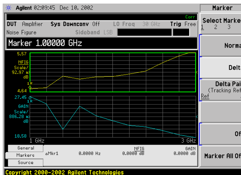
Figure 2-14 The Delta Marker State enabled
