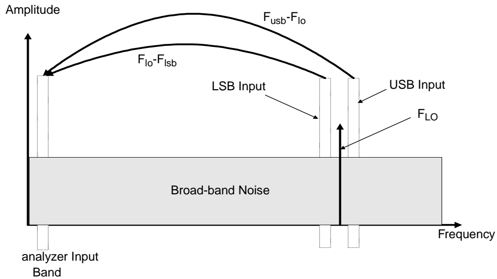
Figure 4-19 DSB System Downconverter Measurements
