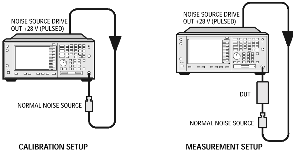
Figure 4-2 PSA Basic Noise Figure Measurement - No Frequency Conversion
