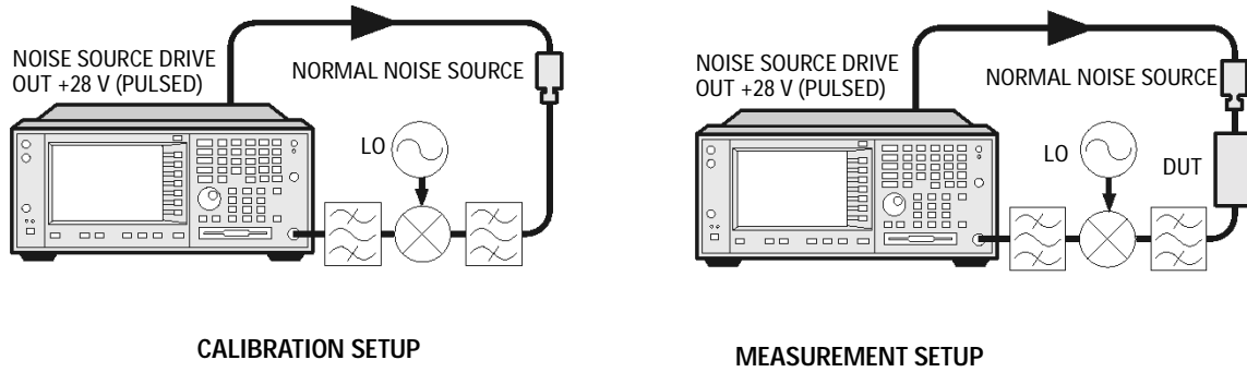
Figure 4-4 Setting Up a PSA for Frequency Converting DUT Measurement
