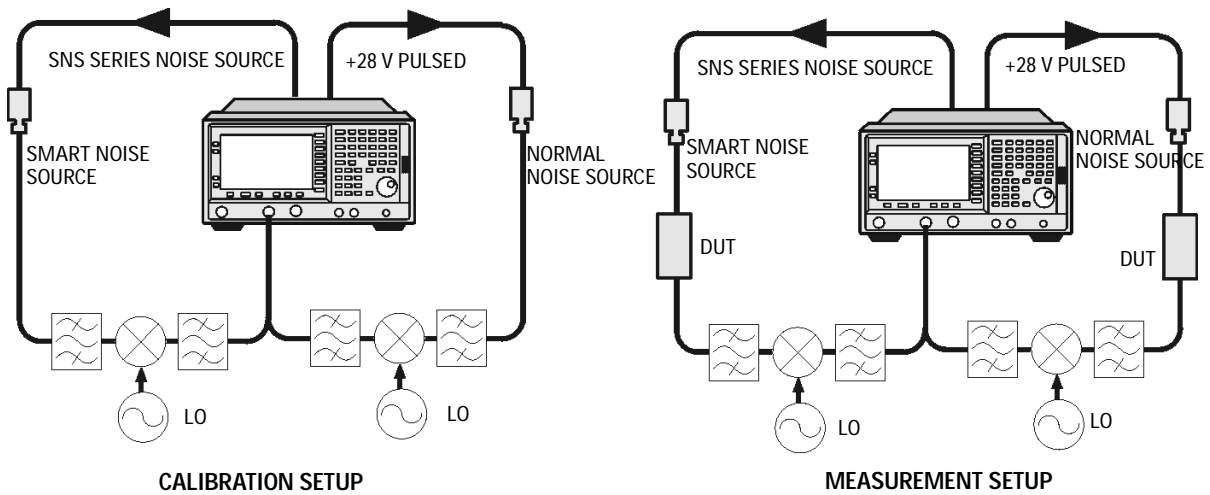
Figure 4-18 PSA System Downconverter Calibration and Measurement
