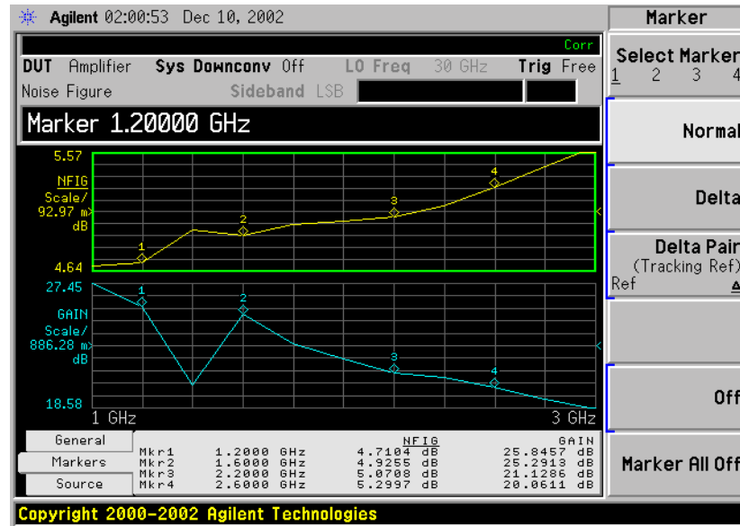
Figure 2-13 Four Normal State Markers
