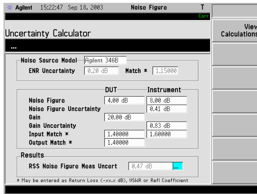
Figure 3-11 Noise Figure Uncertainty Calculator Screen
