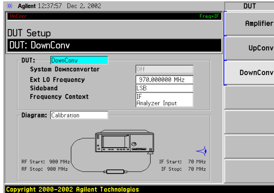
Figure 4-12 DUT Setup Form
