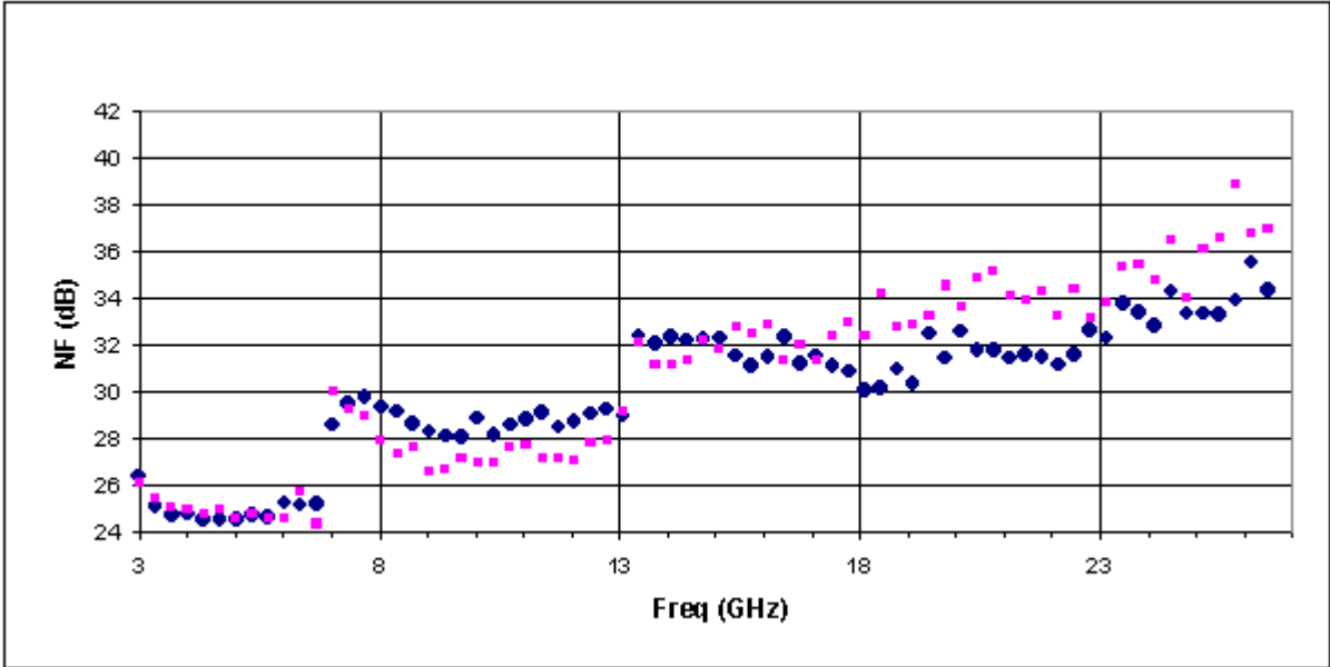
Figure 8-6 No Preamp - Nominal Noise Figure 1
