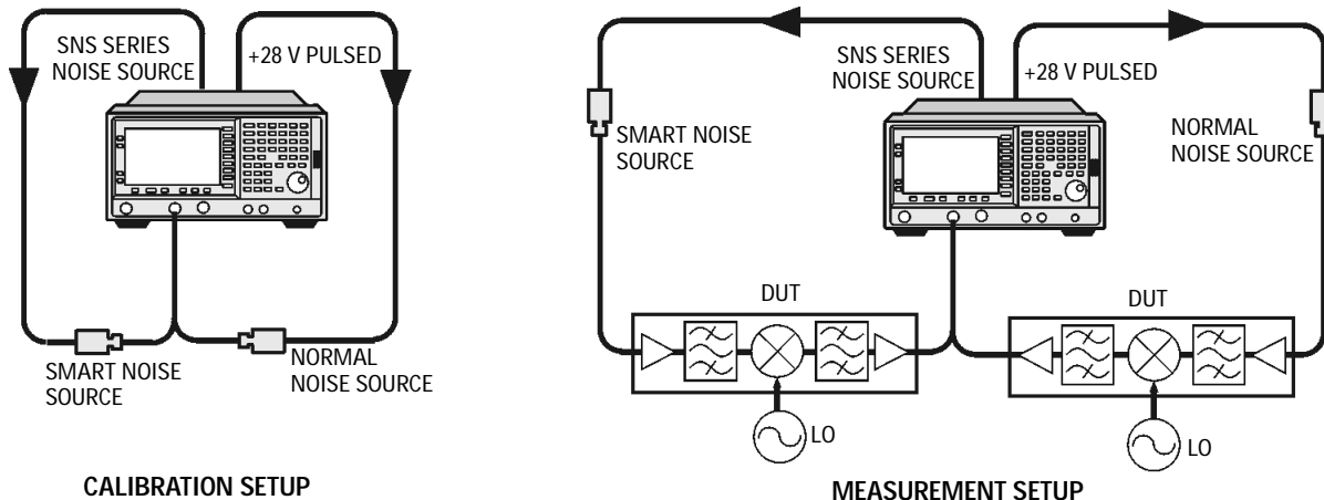
Figure 4-5 ESA Frequency Converting DUT Measurement
